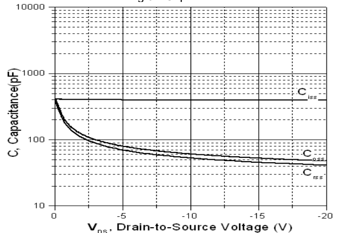
Fig.6 - Capacitance
