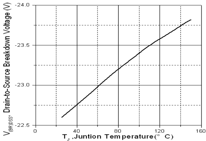
Fig.3 - Drain-to-Source Breakdown Voltage vs. Junction Temperature
