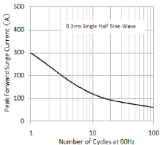
Figure 3. Maximum Non-Repetitive Peak Forward Surge Current
