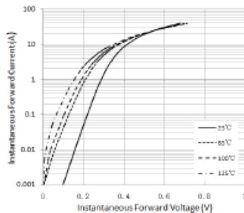
Figure 2. Typical Instantaneous Forward Characteristics
