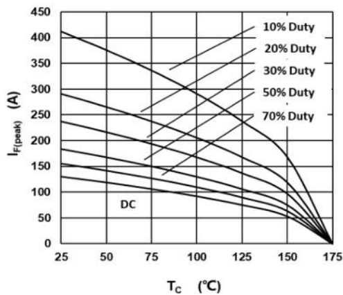
Fig.3 –Current Derating
