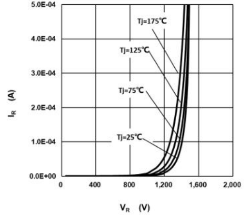
Fig.2 –Reverse Characteristics
