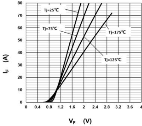
Fig.1 –Forward Characteristics
