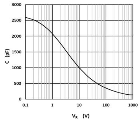
Fig.4 –Capacitance vs. Reverse Voltage
