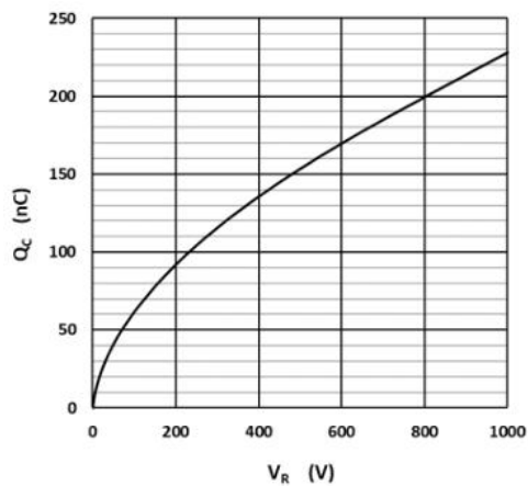
Fig.5 –Total Capacitance Charge vs. Reverse Voltage
