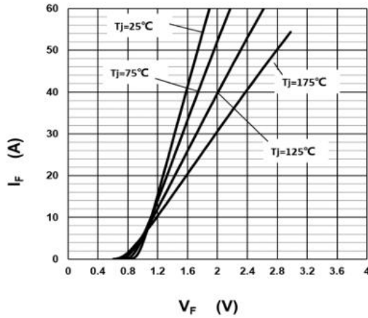
Fig.1 –Forward Characteristics
