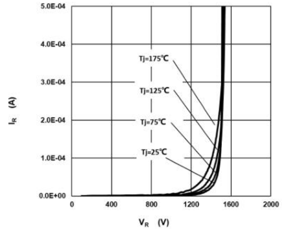
Fig.2 –Reverse Characteristics
