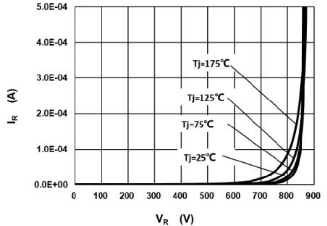
Fig.2 –Reverse Characteristics
