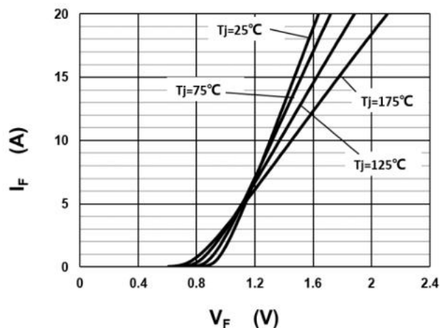
Fig.1 –Forward Characteristics
