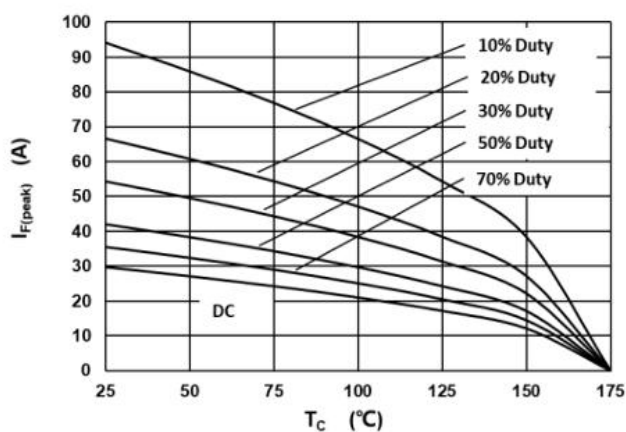
Fig.3 –Current Derating
