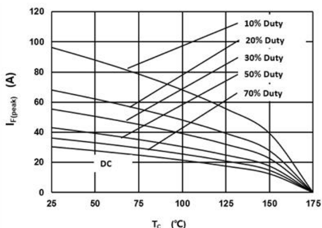
Fig.3 –Current Derating
