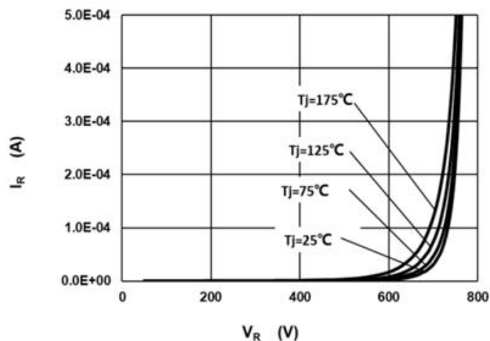
Fig.2 –Reverse Characteristics
