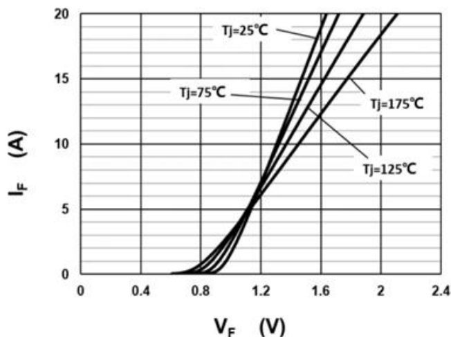
Fig.1 –Forward Characteristics
