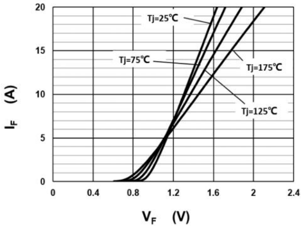
Fig.1 –Forward Characteristics
