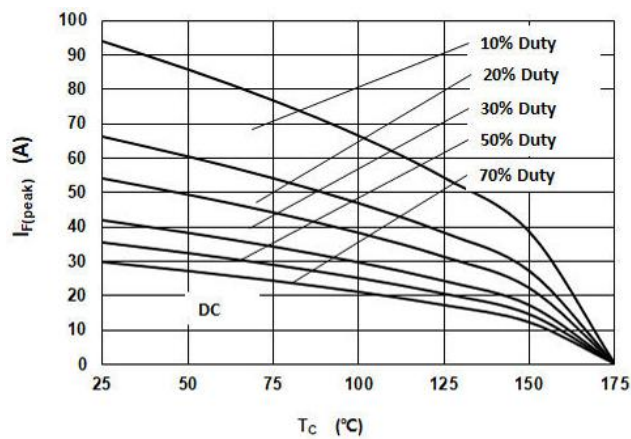
Fig.3 –Current Derating
