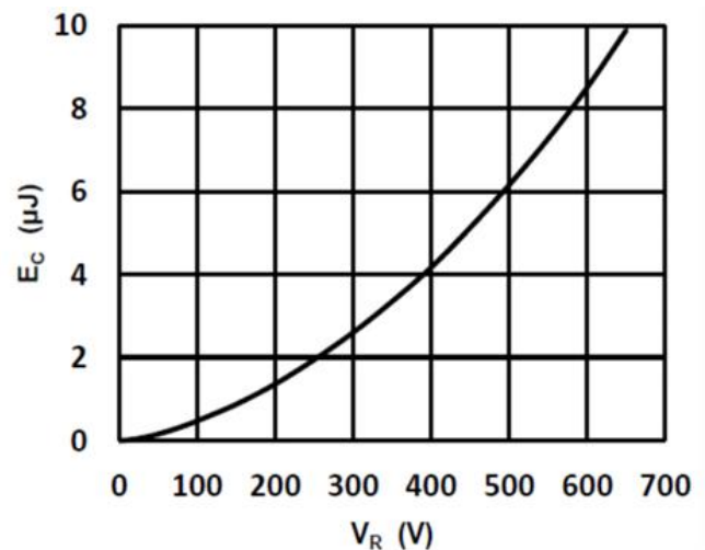
Fig.6 –Typical Capacitance Stored Energy
