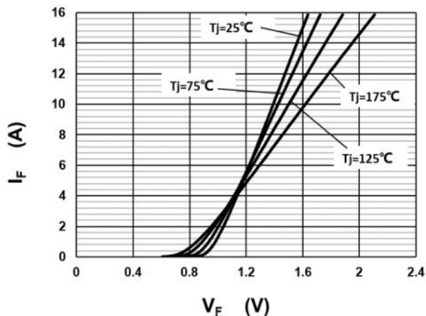
Fig.1 –Forward Characteristics
