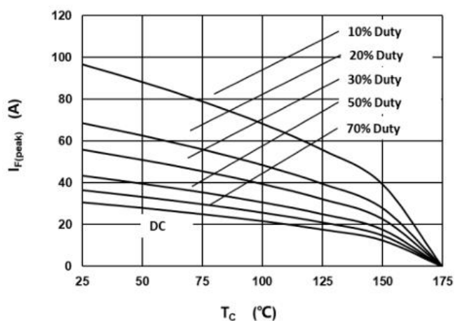
Fig.3 –Current Derating
