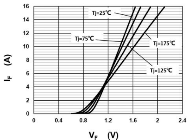
Fig.1 –Forward Characteristics
