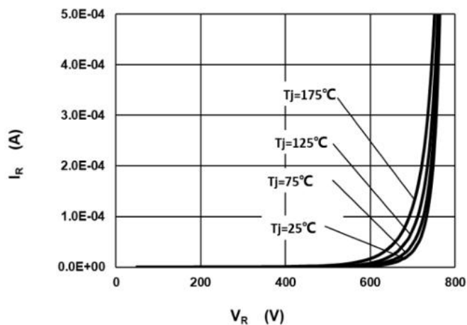
Fig.2 –Reverse Characteristics
