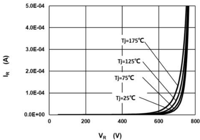
Fig.2 –Reverse Characteristics
