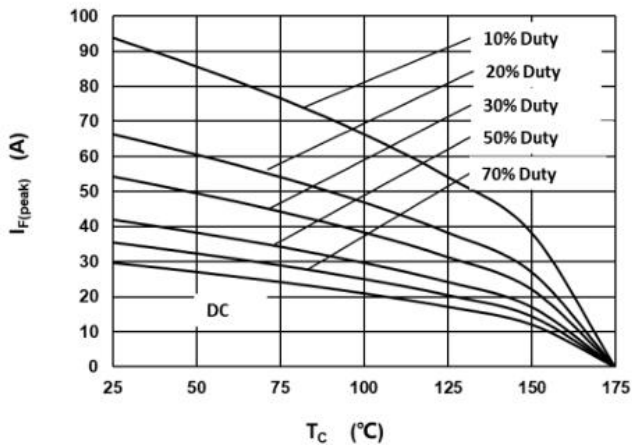
Fig.3 –Current Derating
