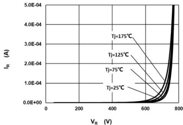
Fig.2 –Reverse Characteristics
