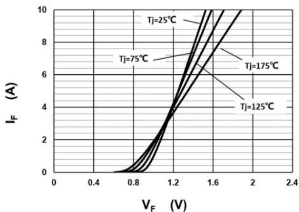
Fig.1 –Forward Characteristics
