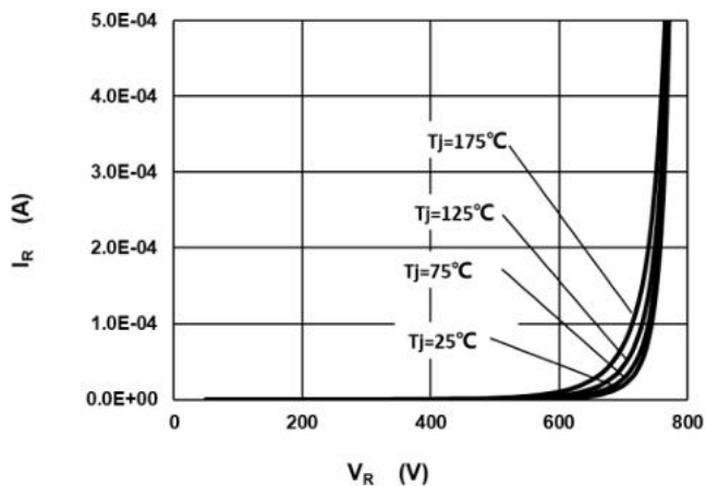
Fig.2 –Reverse Characteristics
