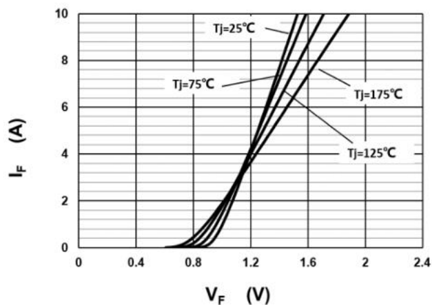
Fig.1 –Forward Characteristics
