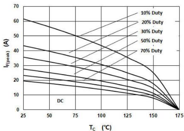
Fig.3 –Current Derating
