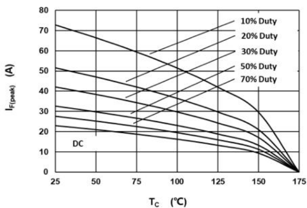
Fig.3 –Current Derating
