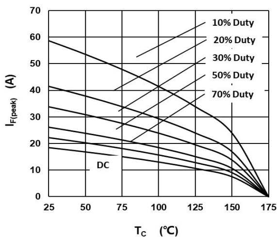
Fig.3 –Current Derating
