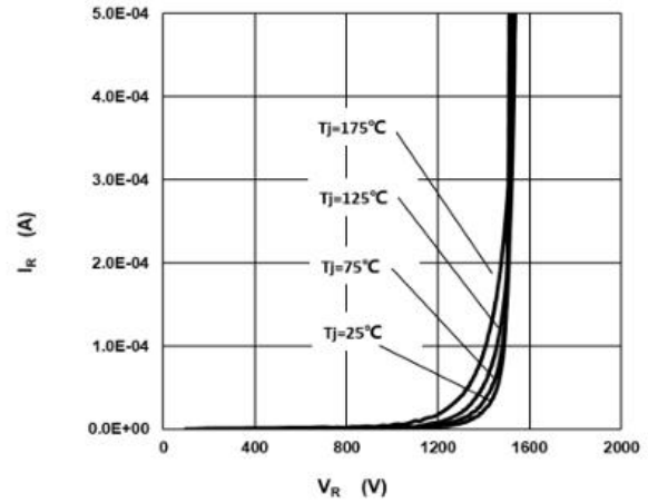
Fig.2 –Reverse Characteristics
