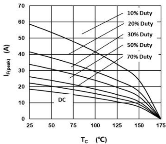
Fig.3 –Current Derating
