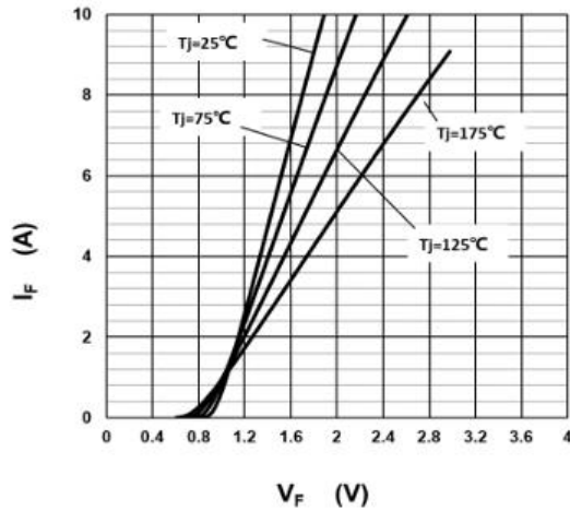
Fig.1 –Forward Characteristics
