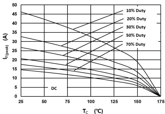
Fig.3 –Current Derating
