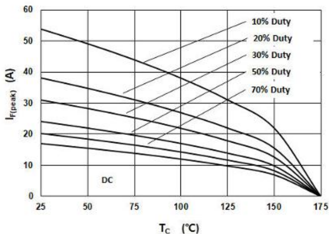
Fig.3 –Current Derating
