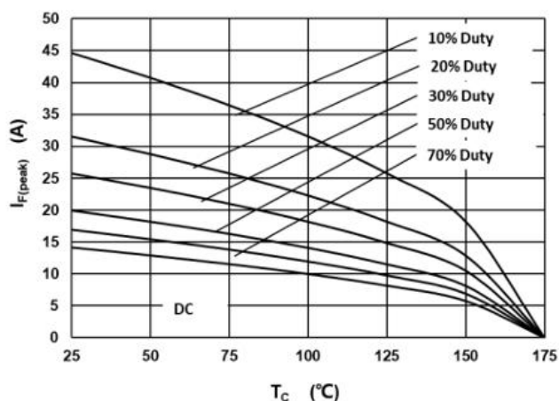
Fig.3 –Current Derating
