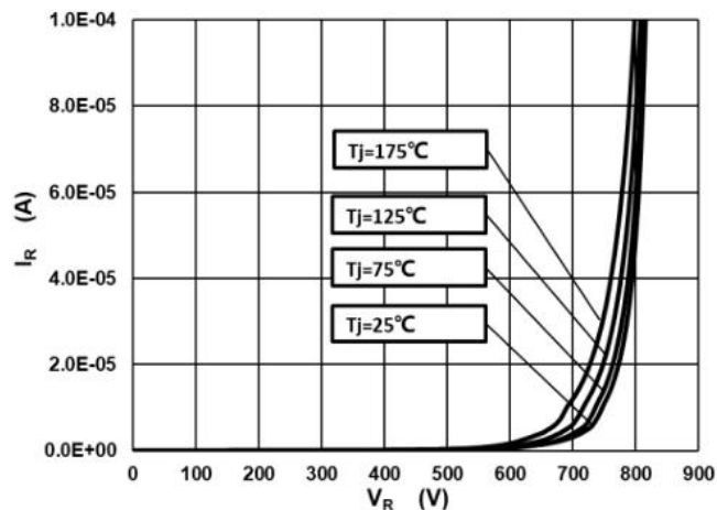
Fig.2 –Reverse Characteristics
