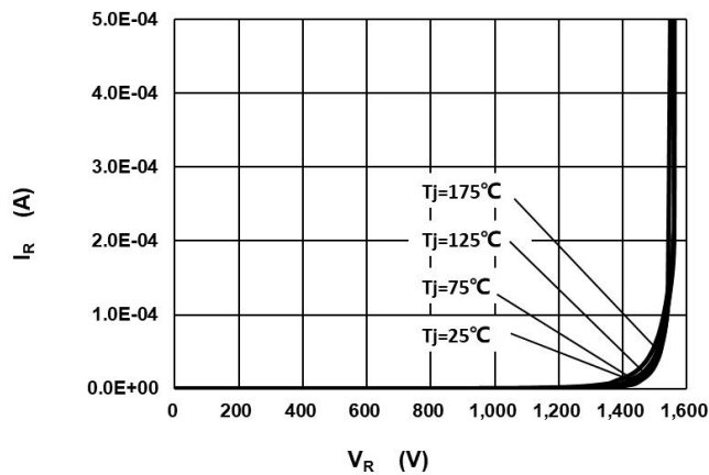
Fig.2 –Reverse Characteristics
