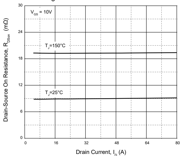
Fig. 3 - Drain-Source On-Resistance
