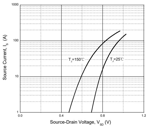
Fig. 9 - Forward Characteristic
