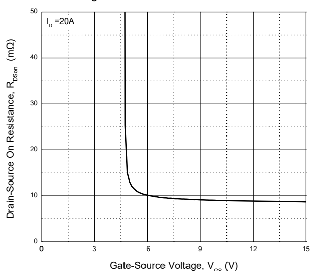
Fig. 5 - Drain-Source On-Resistance
