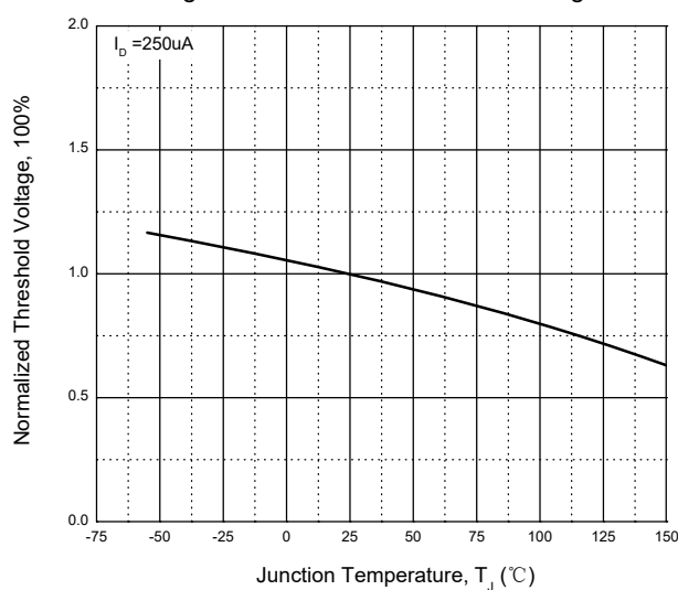
Fig. 6 - Normalized Threshold Voltage
