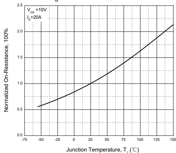
Fig. 4 - Normalized On-Resistance
