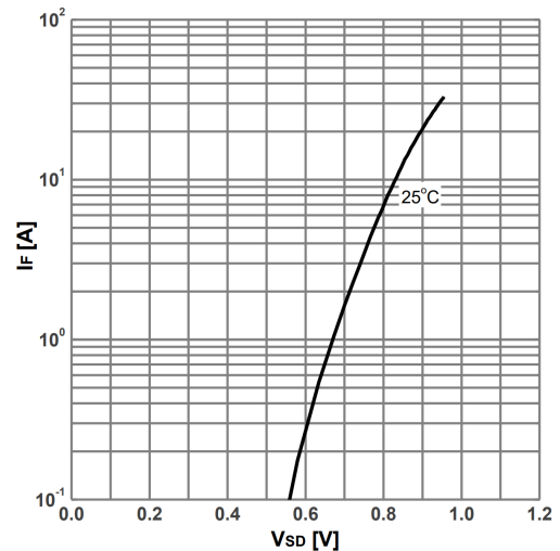
Fig.6 - Forward Characteristic
