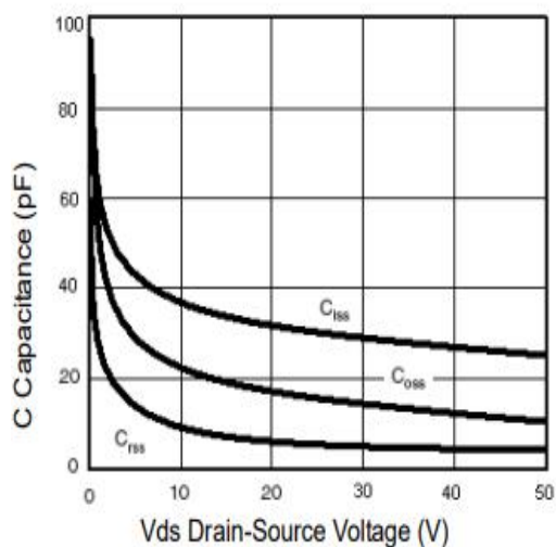
Fig.5 - Capacitance
