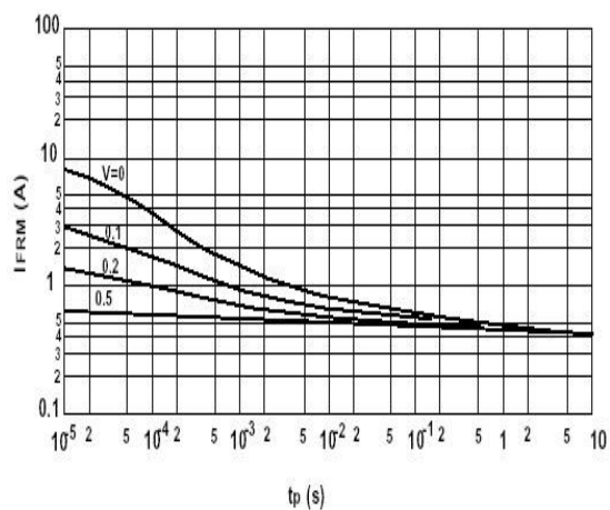
Admissible repetitive peak forward current VS. pulse duration
